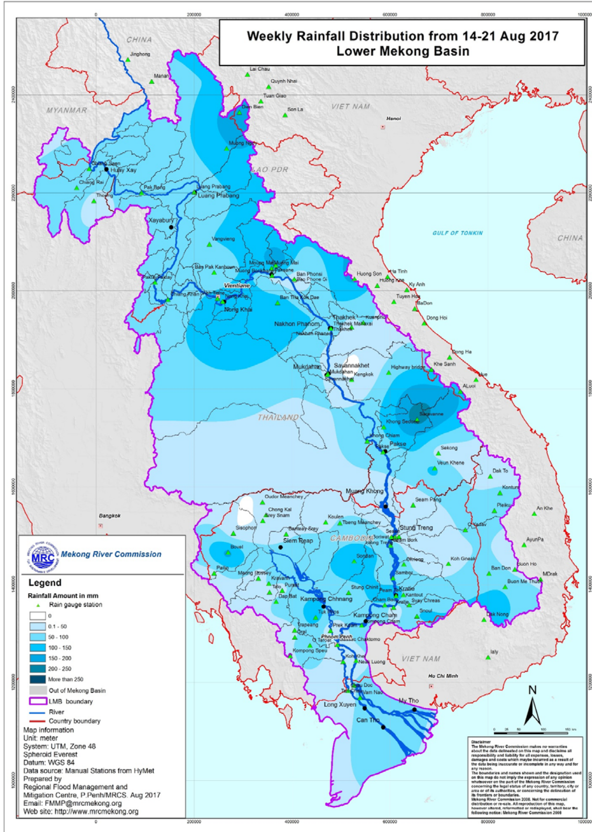
Figure 2: Weekly Rainfall Distribution over the LMB from 14 th – 21 st August 2017
