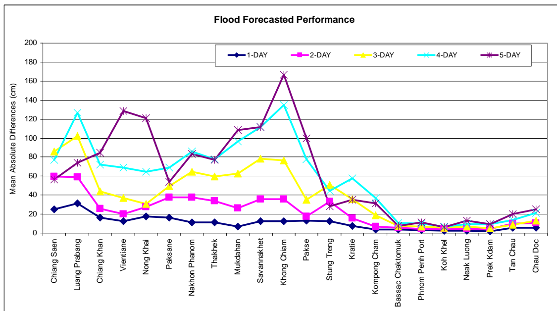
Figure B1: Average flood forecast accuracy along the Mekong mainstream (from 14 th – 21 st August 2017)
