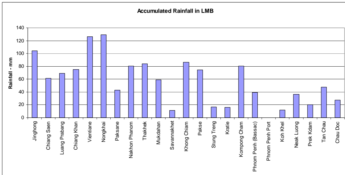
Figure 1: Accumulated Rainfall Distribution over the LMB from 14 th – 21 st August 2017
